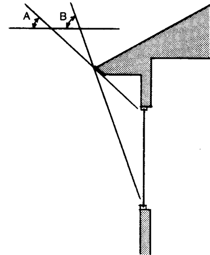
South Overhang Sizing In Nashville, an ideally sized south overhang should allow full exposure of the window when the sun has a noon altitude of 35 degrees (angle A) and fully shade the window when the sun has a noon altitude of 72 degrees (angle B).
