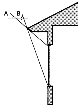
South Overhang Sizing In Little Rock, an ideally sized south overhang should allow full exposure of the window when the sun has a noon altitude of 36 degrees (angle A) and fully shade the window when the sun has a noon altitude of 73 degrees (angle B).
