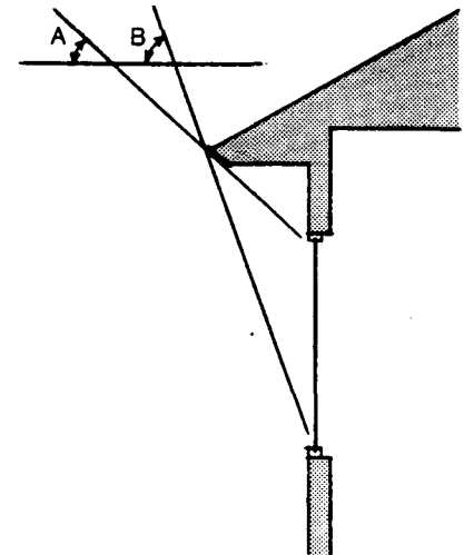
South Overhang Sizing In Ft. Huachuca, an ideally sized south overhang should allow full exposure of the window when the sun has a noon altitude of 39 degrees (angle A) and fully shade the window when the sun has a noon altitude of 76 degrees (angle B).
