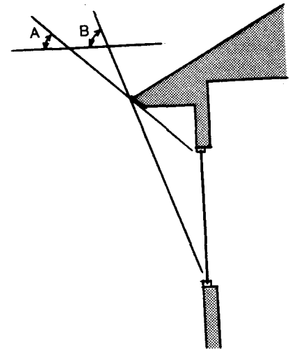
South Overhang Sizing In Fresno, an ideally sized south overhang should allow full exposure of the window when the sun has a noon altitude of 34 degrees (angle A) and fully shade the window when the sun has a noon altitude of 71 degrees (angle B).
