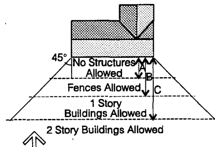
Ideal Solar Access Buildings, trees or other obstructions should not be located so as to shade the south wall of solar buildings. At this latitude, A = 9 ft., B = 16 ft., and C = 37 ft.
