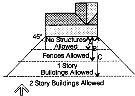
Ideal Solar Access Buildings, trees or other obstructions should not be located so as to shade the south wall of solar buildings. At this latitude, A = 15 ft., B = 26 ft., and C = 59 ft.
