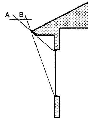
South Overhang Sizing In Mount Shasta, an ideally sized south overhang should allow full exposure of the window when the sun has a noon altitude of 30 degrees (angle A) and fully shade the window when the sun has a noon altitude of 67 degrees (angle B).
