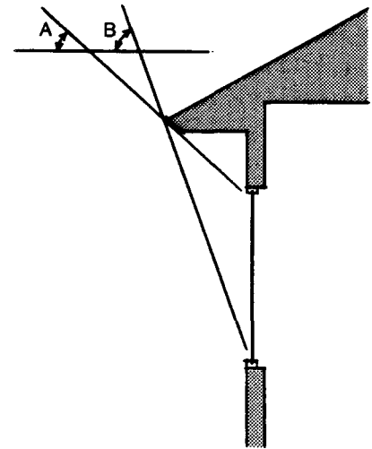
South Overhang Sizing In Oakland, an ideally sized south overhang should allow full exposure of the window when the sun has a noon altitude of 33 degrees (angle A) and fully shade the window when the sun has a noon altitude of 70 degrees (angle B).
