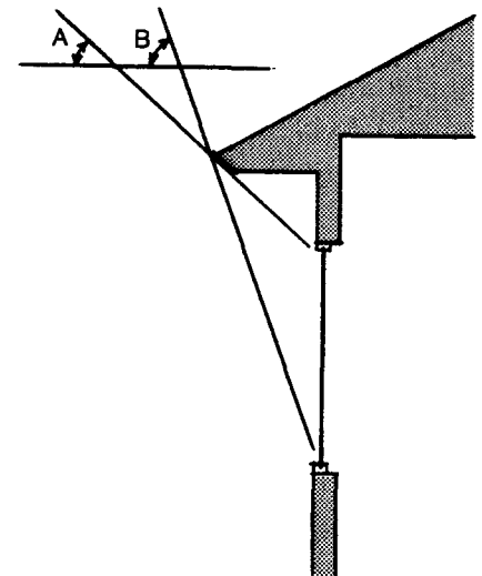
South Overhang Sizing In Lake Tahoe Mountain Region, an ideally sized south overhang should allow full exposure of the window when the sun has a noon altitude of 30 degrees (angle A) and fully shade the window when the sun has a noon altitude of 67 degrees (angle B).
