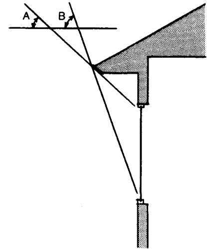
South Overhang Sizing In Grand Junction, an ideally sized south overhang should allow full exposure of the window when the sun has a noon altitude of 32 degrees (angle A) and fully shade the window when the sun has a noon altitude of 69 degrees (angle B).
