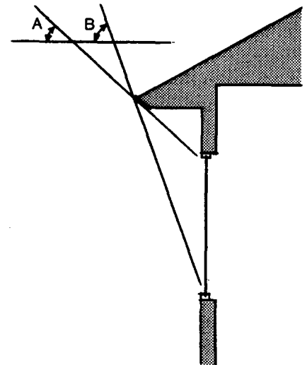
South Overhang Sizing In Steamboat Springs, an ideally sized south overhang should allow full exposure of the window when the sun has a noon altitude of 31 degrees (angle A) and fully shade the window when the sun has a noon altitude of 68 degrees (angle B).
