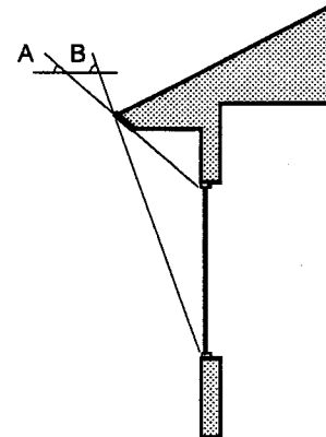
South Overhang Sizing In Carbondale, an ideally sized south overhang should allow full exposure of the window when the sun has a noon altitude of 31 degrees (angle A) and fully shade the window when the sun has a noon altitude of 68 degrees (angle B).
