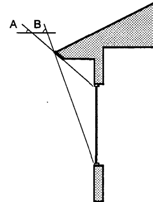
South Overhang Sizing In Burlington, an ideally sized south overhang should allow full exposure of the window when the sun has a noon altitude of 30 degrees (angle A) and fully shade the window when the sun has a noon altitude of 67 degrees (angle B).
