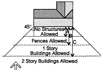
Ideal Solar Access Buildings, trees or other obstructions should not be located so as to shade the south wall of solar buildings. At this latitude, A = 13 ft., B = 23 ft., and C = 53 ft.
