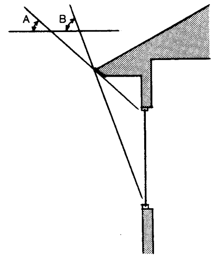
South Overhang Sizing In Evansville, an ideally sized south overhang should allow full exposure of the window when the sun has a noon altitude of 33 degrees (angle A) and fully shade the window when the sun has a noon altitude of 70 degrees (angle B).
