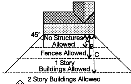
Ideal Solar Access Buildings, trees or other obstructions should not be located so as to shade the south wall of solar buildings. At this latitude, A = 12 ft., B = 21 ft., and C = 47 ft.
