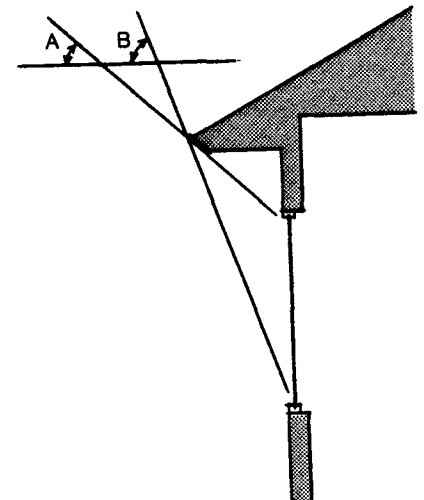
South Overhang Sizing In Western, an ideally sized south overhang should allow full exposure of the window when the sun has a noon altitude of 35 degrees (angle A) and fully shade the window when the sun has a noon altitude of 72 degrees (angle B).
