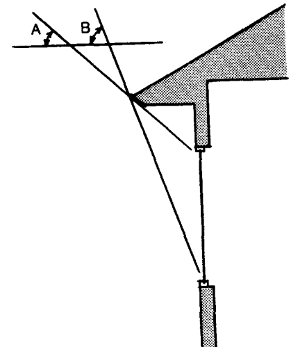
South Overhang Sizing In Patuxent River, an ideally sized south overhang should allow full exposure of the window when the sun has a noon altitude of 33 degrees (angle A) and fully shade the window when the sun has a noon altitude of 70 degrees (angle B).
