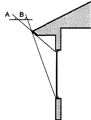
South Overhang Sizing In Caribou, an ideally sized south overhang should allow full exposure of the window when the sun has a noon altitude of 24 degrees (angle A) and fully shade the window when the sun has a noon altitude of 61 degrees (angle B).
