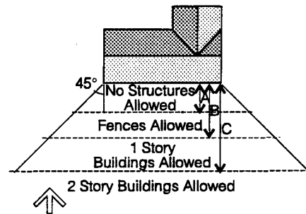
Ideal Solar Access Buildings, trees or other obstructions should not be located so as to shade the south wall of solar buildings. At this latitude, A = 25 ft., B = 43 ft., and C = 99 ft.
