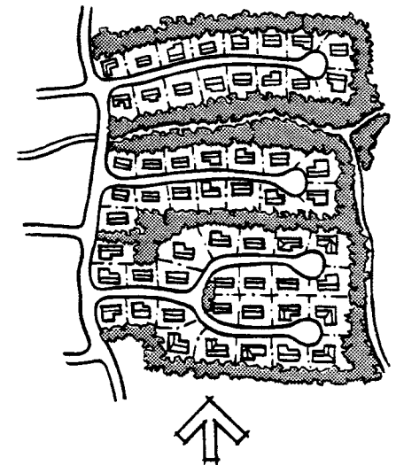
Solar Subdivision Layouts Solar access may be provided to the rear yard, the side yard or the front yard of solar homes.
