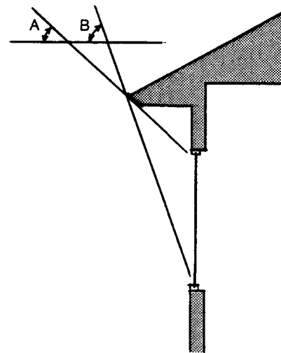
South Overhang Sizing In Grand Rapids, an ideally sized south overhang should allow full exposure of the window when the sun has a noon altitude of 28 degrees (angle A) and fully shade the window when the sun has a noon altitude of 65 degrees (angle B).
