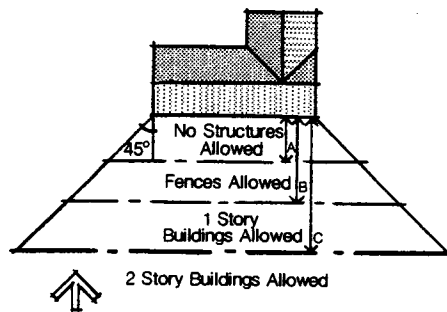
Ideal Solar Access Buildings, trees or other obstructions should not be located so as to shade the south wall of solar buildings. At this latitude, A = 17 ft., B = 29 ft., and C = 67 ft.
