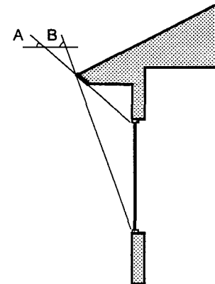
South Overhang Sizing In Billings, an ideally sized south overhang should allow full exposure of the window when the sun has a noon altitude of 25 degrees (angle A) and fully shade the window when the sun has a noon altitude of 62 degrees (angle B).
