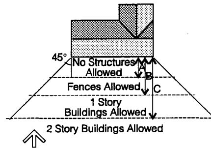
Ideal Solar Access Buildings, trees or other obstructions should not be located so as to shade the south wall of solar buildings. At this latitude, A = 22 ft., B = 38 ft., and C = 88 ft.
