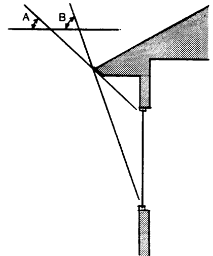
South Overhang Sizing In Cut Bank, an ideally sized south overhang should allow full exposure of the window when the sun has a noon altitude of 22 degrees (angle A) and fully shade the window when the sun has a noon altitude of 59 degrees (angle B).
