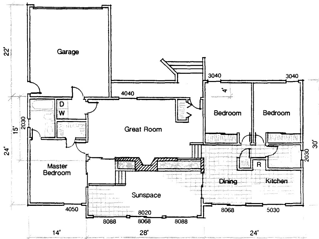
Floor Plan
