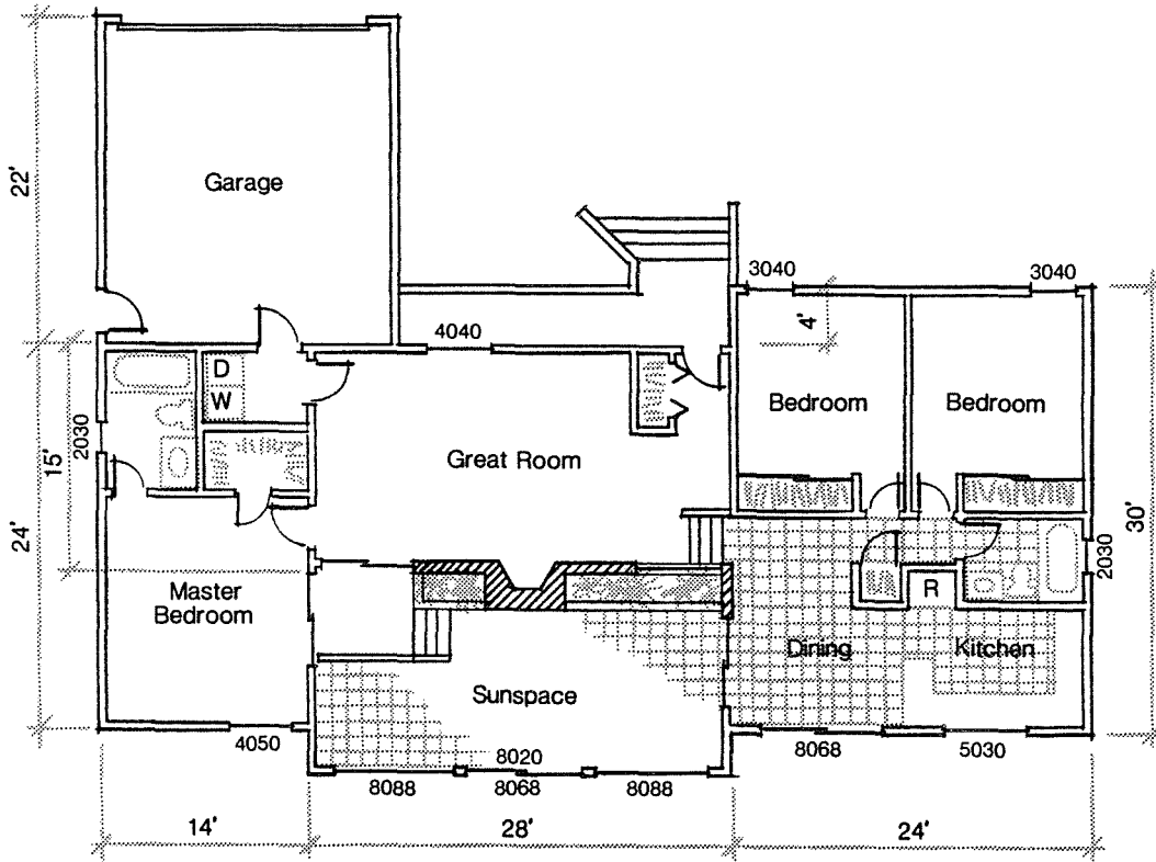
Floor Plan
