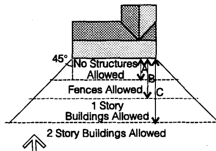
Ideal Solar Access Buildings, trees or other obstructions should not be located so as to shade the south wall of solar buildings. At this latitude, A = 10 ft., B = 18 ft., and C = 42 ft.
