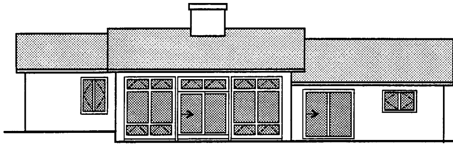
SOUTH ELEVATION
