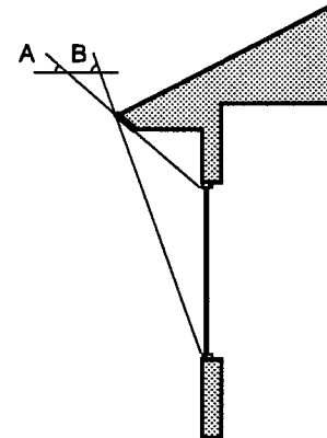
South Overhang Sizing In North Platte, an ideally sized south overhang should allow full exposure of the window when the sun has a noon altitude of 30 degrees (angle A) and fully shade the window when the sun has a noon altitude of 67 degrees (angle B).
