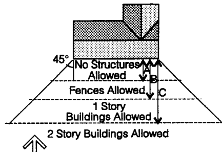
Ideal Solar Access Buildings, trees or other obstructions should not be located so as to shade the south wall of solar buildings. At this latitude, A = 15 ft., B = 25 ft., and C = 58 ft.
