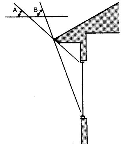
South Overhang Sizing In Scottsbluff, an ideally sized south overhang should allow full exposure of the window when the sun has a noon altitude of 29 degrees (angle A) and fully shade the window when the sun has a noon altitude of 66 degrees (angle B).
