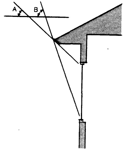
South Overhang Sizing In Lordsburg, an ideally sized south overhang should allow full exposure of the window when the sun has a noon altitude of 39 degrees (angle A) and fully shade the window when the sun has a noon altitude of 76 degrees (angle B).
