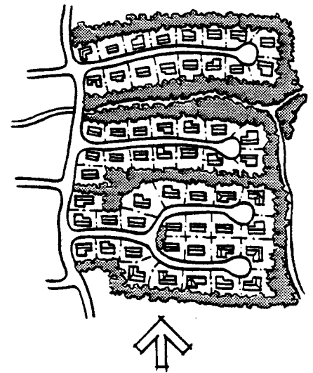
Solar Subdivision Layouts Short east-west cul-de-sacs tied into north-south collectors is a good street pattern for solar access.
