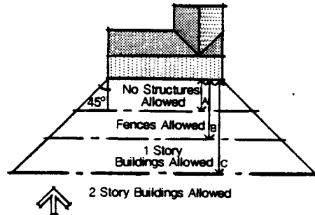
Ideal Solar Access Buildings, trees or other obstructions should not be located so as to shade the south wall of solar buildings. At this latitude, A = 8 ft., B = 14 ft., and C = 33 ft.
