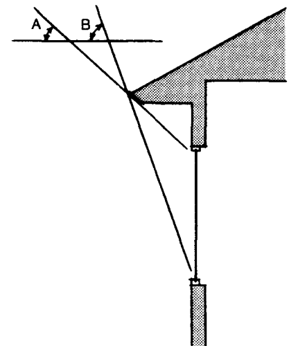
South Overhang Sizing In Roswell, an ideally sized south overhang should allow full exposure of the window when the sun has a noon altitude of 38 degrees (angle A) and fully shade the window when the sun has a noon altitude of 75 degrees (angle B).
