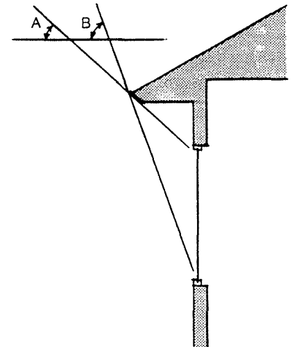
South Overhang Sizing In Santa Fe, an ideally sized south overhang should allow full exposure of the window when the sun has a noon altitude of 36 degrees (angle A) and fully shade the window when the sun has a noon altitude of 73 degrees (angle B).
