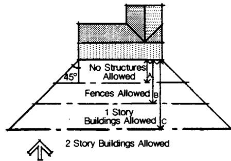
Ideal Solar Access Buildings, trees or other obstructions should not be located so as to shade the south wall of solar buildings. At this latitude, A = 13 ft., B = 23 ft., and C = 52 ft.
