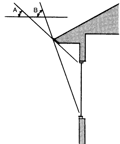
South Overhang Sizing In Reno, an ideally sized south overhang should allow full exposure of the window when the sun has a noon altitude of 32 degrees (angle A) and fully shade the window when the sun has a noon altitude of 69 degrees (angle B).
