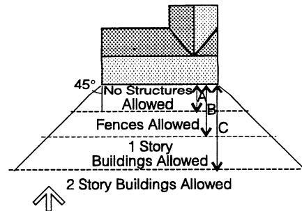
Ideal Solar Access Buildings, trees or other obstructions should not be located so as to shade the south wall of solar buildings. At this latitude, A = 17 ft., B = 29 ft., and C = 66 ft.
