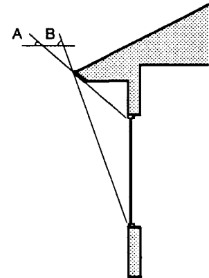
South Overhang Sizing In Binghamton, an ideally sized south overhang should allow full exposure of the window when the sun has a noon altitude of 29 degrees (angle A) and fully shade the window when the sun has a noon altitude of 66 degrees (angle B).
