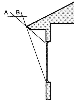
South Overhang Sizing In Buffalo, an ideally sized south overhang should allow full exposure of the window when the sun has a noon altitude of 28 degrees (angle A) and fully shade the window when the sun has a noon altitude of 65 degrees (angle B).
