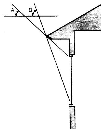
South Overhang Sizing In Akron-Canton, an ideally sized south overhang should allow full exposure of the window when the sun has a noon altitude of 30 degrees (angle A) and fully shade the window when the sun has a noon altitude of 67 degrees (angle B).
