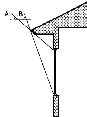
South Overhang Sizing In Philadelphia, an ideally sized south overhang should allow full exposure of the window when the sun has a noon altitude of 31 degrees (angle A) and fully shade the window when the sun has a noon altitude of 68 degrees (angle B).
