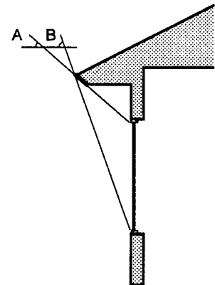
South Overhang Sizing In Wilkes-Barre, an ideally sized south overhang should allow full exposure of the window when the sun has a noon altitude of 30 degrees (angle A) and fully shade the window when the sun has a noon altitude of 67 degrees (angle B).
