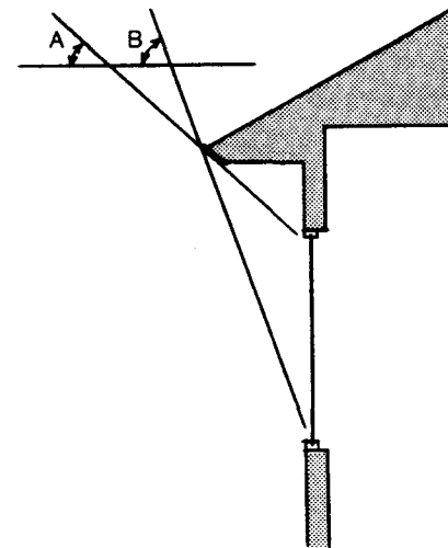
South Overhang Sizing In Memphis, an ideally sized south overhang should allow full exposure of the window when the sun has a noon altitude of 36 degrees (angle A) and fully shade the window when the sun has a noon altitude of 73 degrees (angle B).
