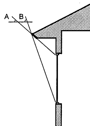
South Overhang Sizing In Abilene, an ideally sized south overhang should allow full exposure of the window when the sun has a noon altitude of 39 degrees (angle A) and fully shade the window when the sun has a noon altitude of 76 degrees (angle B).
