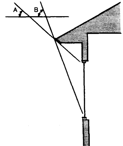
South Overhang Sizing In Corpus Christi, an ideally sized south overhang should allow full exposure of the window when the sun has a noon altitude of 43 degrees (angle A) and fully shade the window when the sun has a noon altitude of 80 degrees (angle B).
