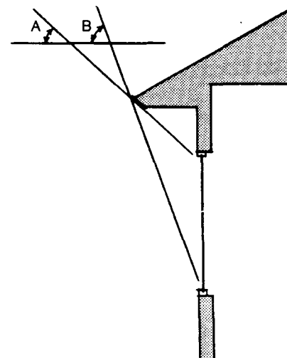
South Overhang Sizing In Lubbock, an ideally sized south overhang should allow full exposure of the window when the sun has a noon altitude of 37 degrees (angle A) and fully shade the window when the sun has a noon altitude of 74 degrees (angle B).
