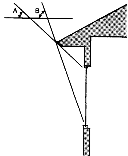
South Overhang Sizing In Fort Worth, an ideally sized south overhang should allow full exposure of the window when the sun has a noon altitude of 38 degrees (angle A) and fully shade the window when the sun has a noon altitude of 75 degrees (angle B).
