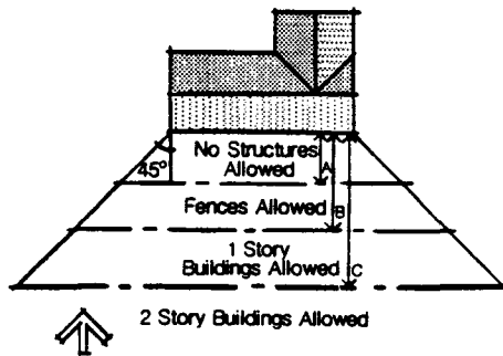
Solar Subdivision Layouts Solar access may be provided to the rear yard, the side yard or the front yard of solar homes.
