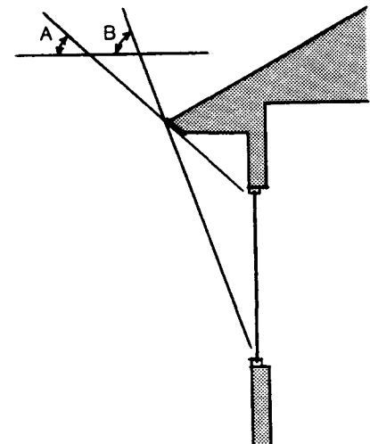
South Overhang Sizing In Bryce Canyon, an ideally sized south overhang should allow full exposure of the window when the sun has a noon altitude of 33 degrees (angle A) and fully shade the window when the sun has a noon altitude of 70 degrees (angle B).
