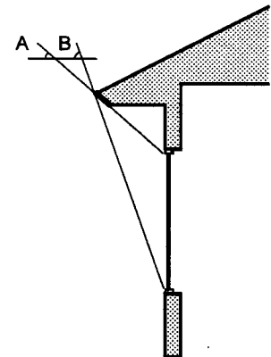
South Overhang Sizing In Norfolk, an ideally sized south overhang should allow full exposure of the window when the sun has a noon altitude of 34 degrees (angle A) and fully shade the window when the sun has a noon altitude of 71 degrees (angle B).
