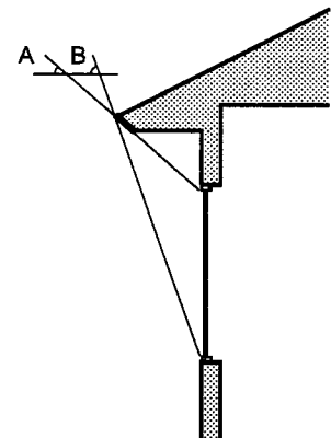
South Overhang Sizing In Shreveport, an ideally sized south overhang should allow full exposure of the window when the sun has a noon altitude of 39 degrees (angle A) and fully shade the window when the sun has a noon altitude of 76 degrees (angle B).
