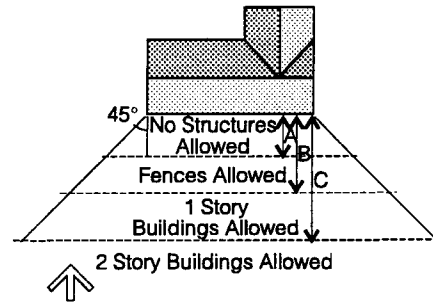
Ideal Solar Access Buildings, trees or other obstructions should not be located so as to shade the south wall of solar buildings. At this latitude, A = 9 ft., B = 15 ft., and C = 34 ft.
