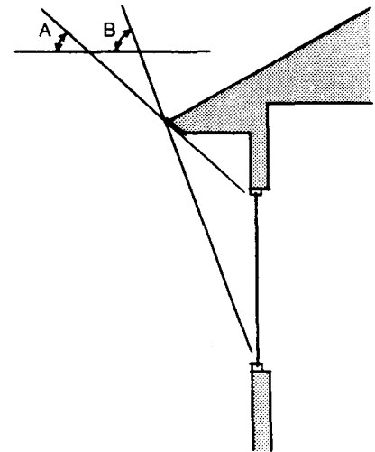
South Overhang Sizing In Olympia, an ideally sized south overhang should allow full exposure of the window when the sun has a noon altitude of 24 degrees (angle A) and fully shade the window when the sun has a noon altitude of 61 degrees (angle B).
