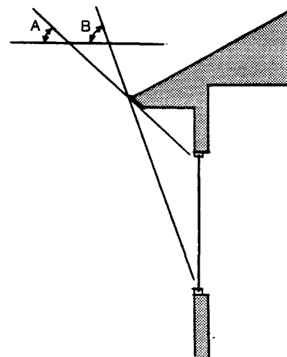
South Overhang Sizing In Milwaukee, an ideally sized south overhang should allow full exposure of the window when the sun has a noon altitude of 28 degrees (angle A) and fully shade the window when the sun has a noon altitude of 65 degrees (angle B).
