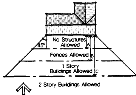
Ideal Solar Access Buildings, trees or other obstructions should not be located so as to shade the south wall of solar buildings. At this latitude, A = 20 ft., B = 35 ft., and C = 79 ft.
