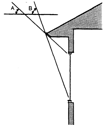
South Overhang Sizing In Sheridan, an ideally sized south overhang should allow full exposure of the window when the sun has a noon altitude of 26 degrees (angle A) and fully shade the window when the sun has a noon altitude of 63 degrees (angle B).
