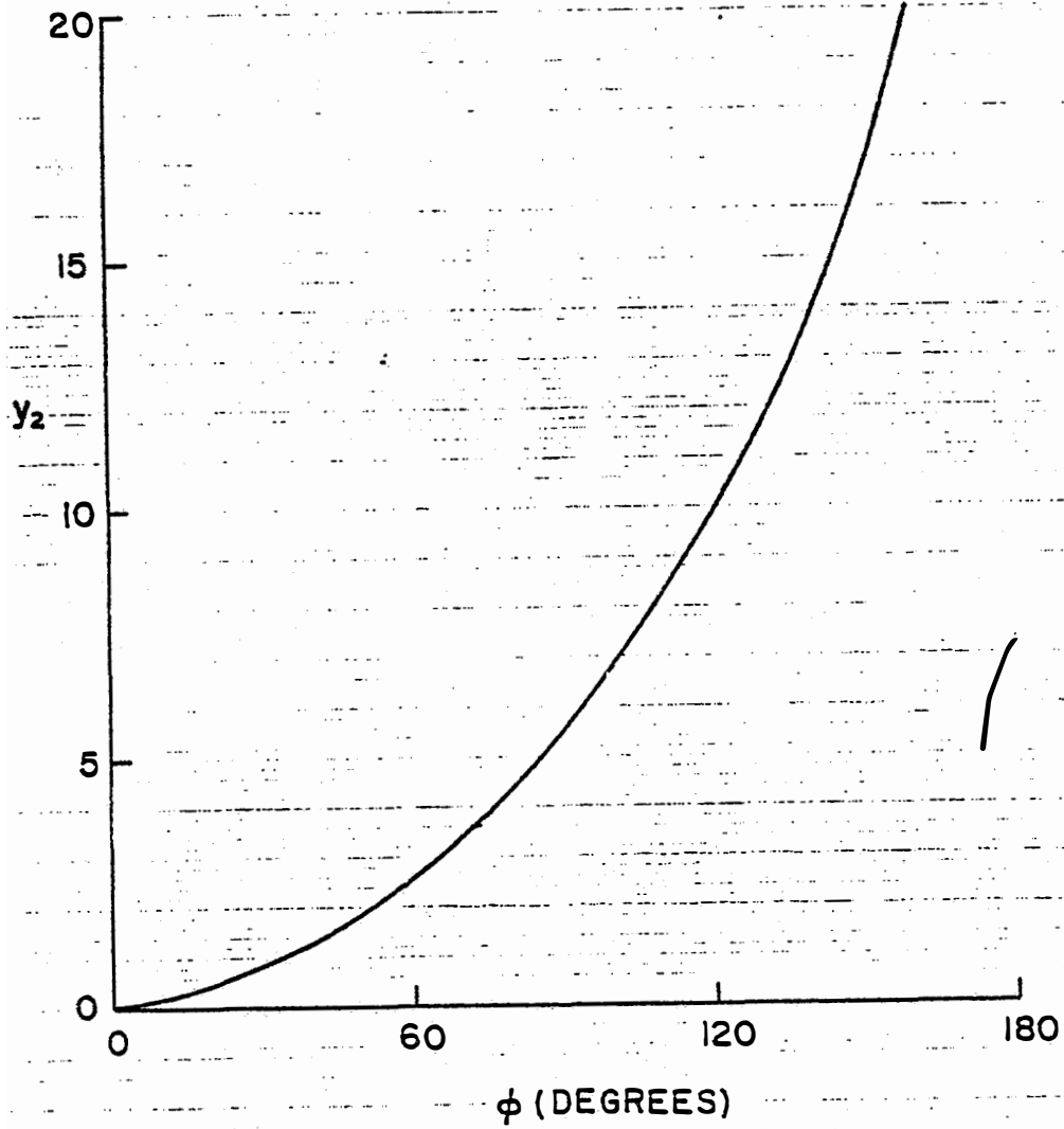
Figure 5: dB level y_2 versus \phi (see equation 15).
