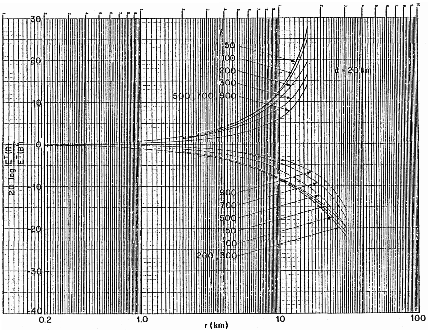
Figure 7(a). Ratio of the direct field strengths at the receiver (R) and WT blade phase center (B) [E^T(R)/E^T(B)] in dB as a function of the distance r from the WT: — \phi = 0 ; - - - \phi = \pi . d = 20 km.
