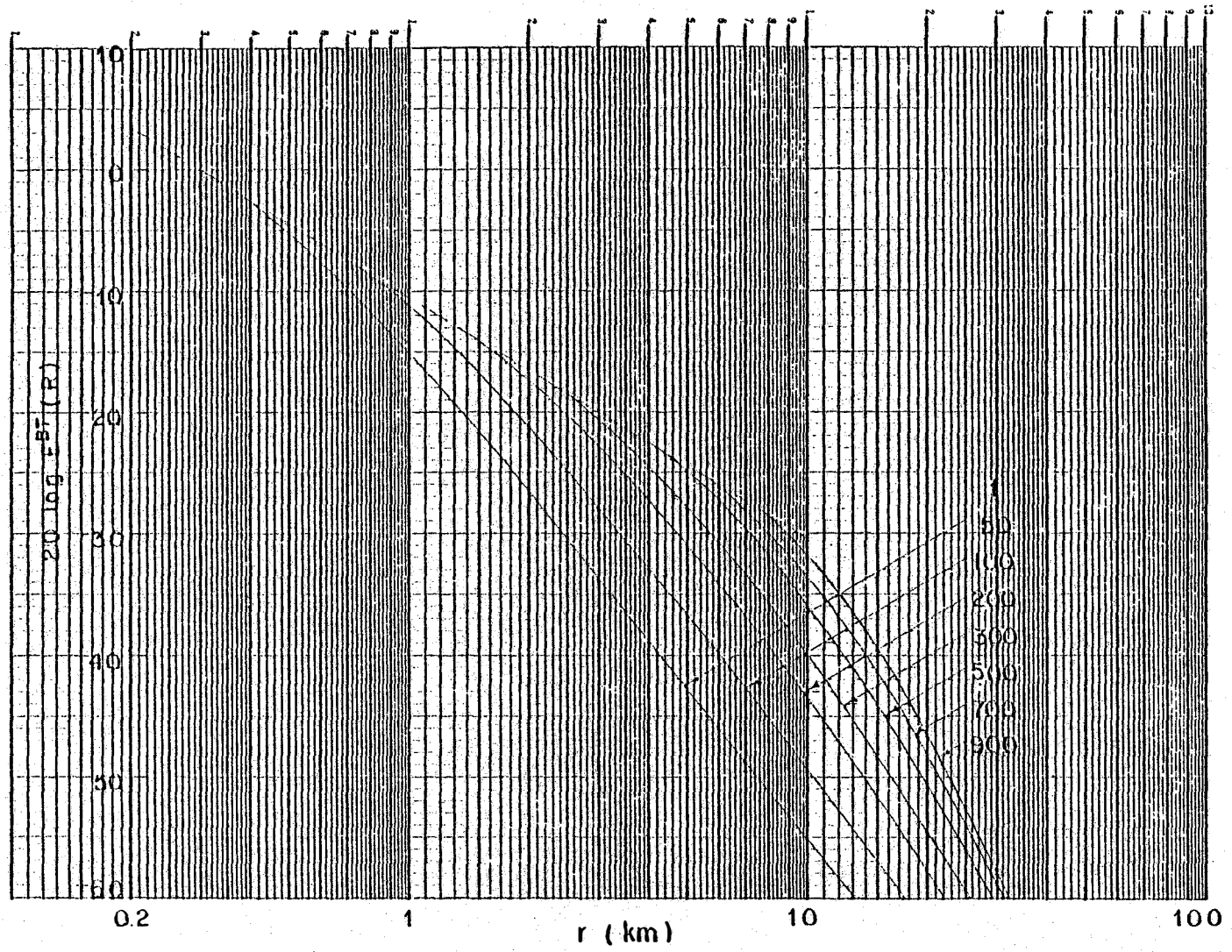
Figure 6(c). Field strength [E^{BT}(r)] in dB above mv/m as a function of distance r from a transmitter located at the WT blade phase center and radiating 1 Kw effective power: h_2 = 10 m, h_3 = 60 m (MOD-2)
