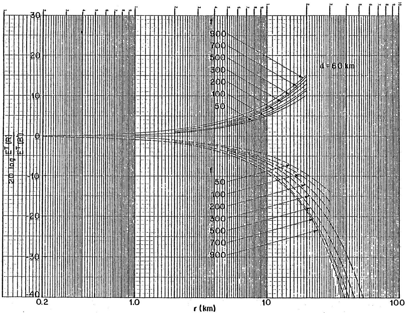
Figure 7(c). Ratio of the direct field strengths at the receiver (R) and WT blade phase center (B) [E^T(R)/E^T(B)] in dB as a function of the distance r from the WT: — \phi = 0 ; - - - \phi = \pi . d = 60 km.
