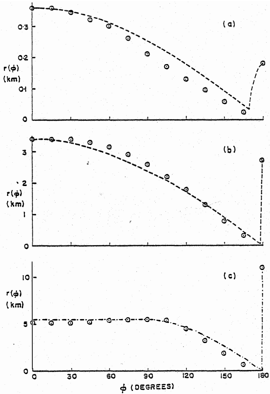
Figure 8. Computed interference zones ( \circ \circ \circ ) for the MOD-1 with d \geq 100 km and (a) f = 50 MHz, (b) f = 500 MHz, (c) f = 900 MHz; --- type A zone, -.-.- type B zone.
