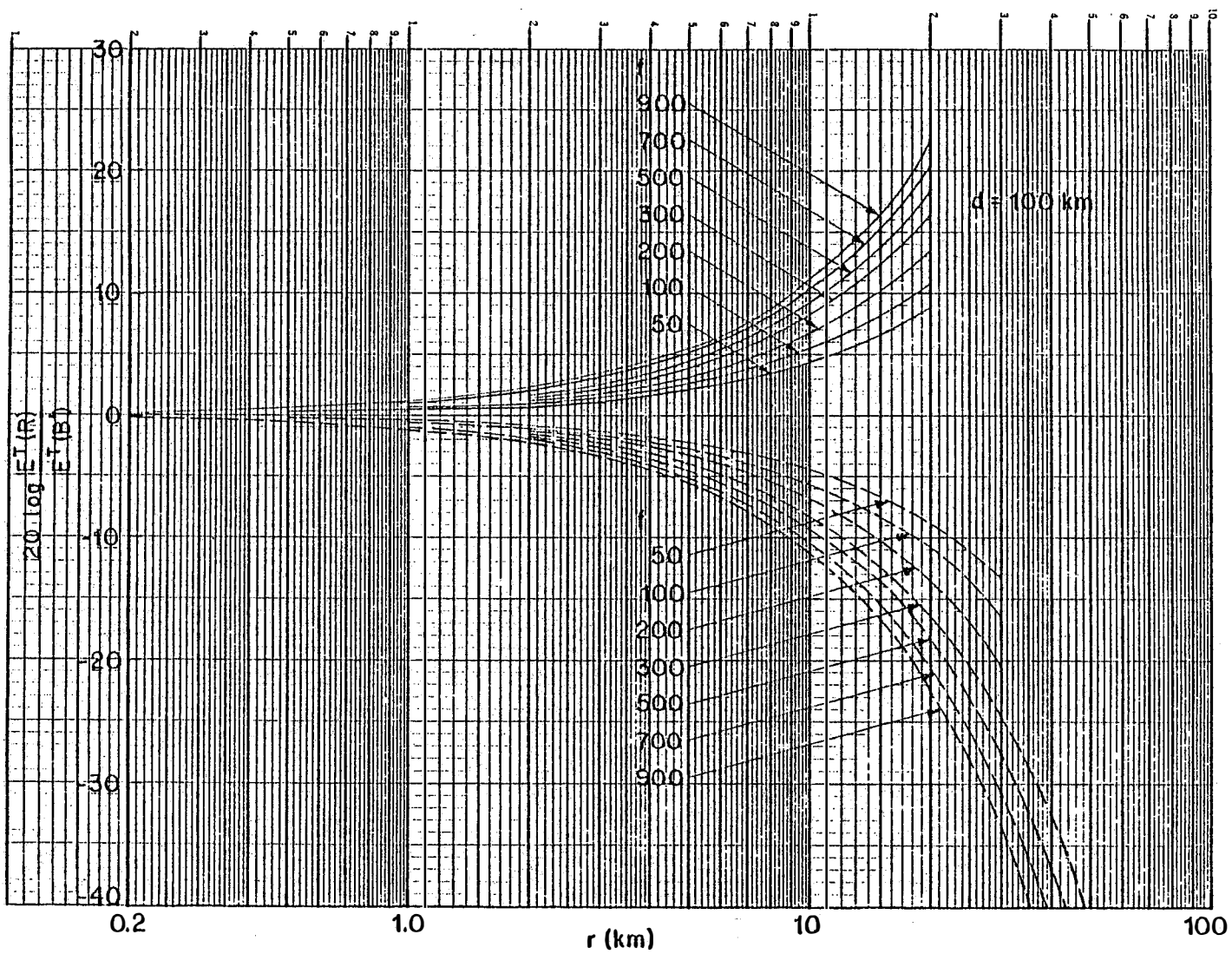
Figure 7(e). Ratio of the direct field strengths at the receiver (R) and WT blade phase center B [E^T(R)/E^T(B)] in dB as a function of the distance r from the WT: — \phi = 0 ; - - - \phi = \pi . d \geq 100 km.
