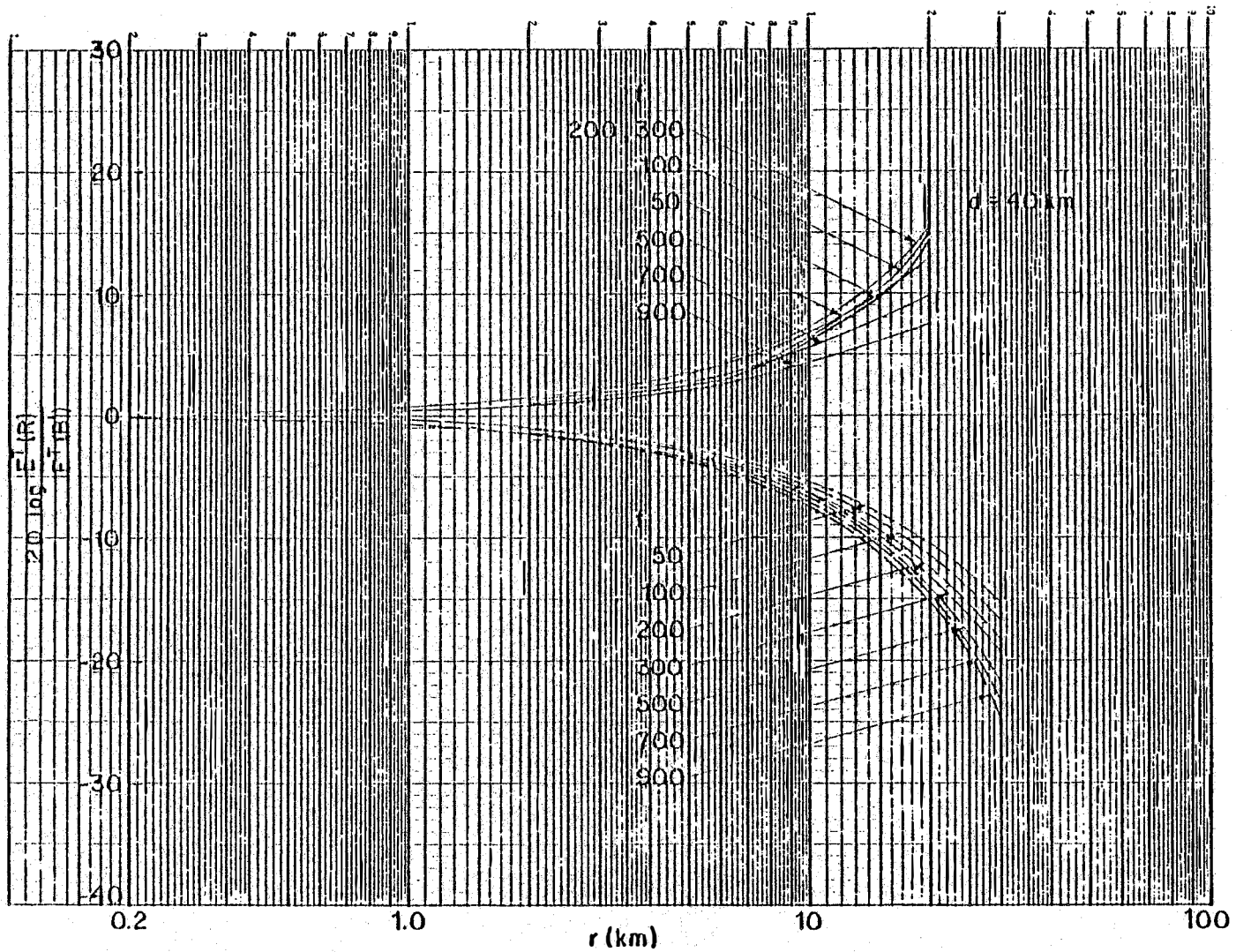
Figure 7(b). Ratio of the direct field strengths at the receiver (R) and WT, blade phase center (B) [E^T(R)/E^T(B)] in dB as a function of the distance r from the WT: — \phi = 0 ; - - - \phi = \pi . d = 40 \text{ km} .
