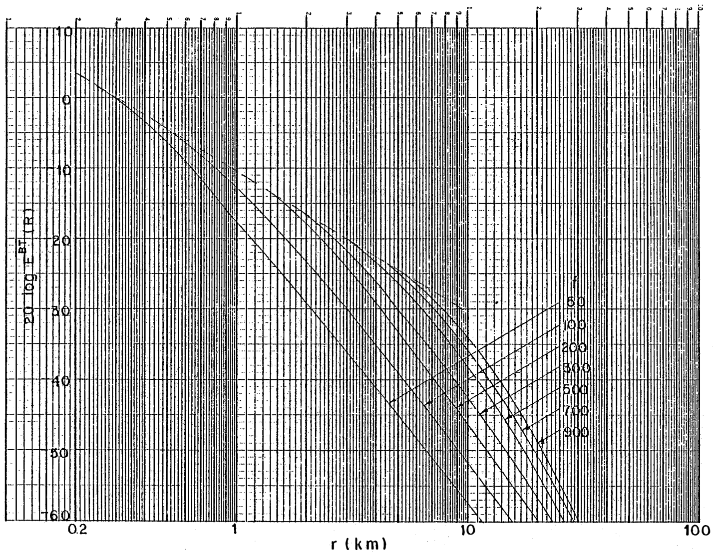
Figure 6(b). Field strength [E^{BT}(R)] in dB above mv/m as a function of distance r from a transmitter located at the WT blade phase center and radiating 1 Kw effective power: h_2 = 10 m, h_3 = 45 m (MOD-1)
