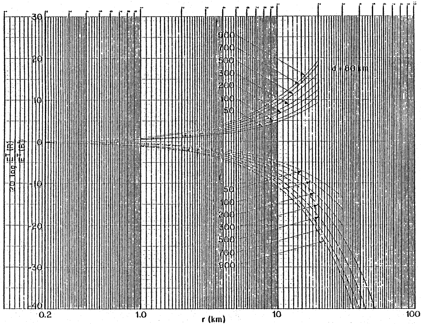
Figure 7(d). Ratio of the direct field strengths at the receiver (R) and WT blade phase center (B) [E^T(R)/E^T(B)] in dB as a function of the distance r from the WT: — \phi = 0 ; - - - \phi = \pi . d = 80 \text{ km} .
