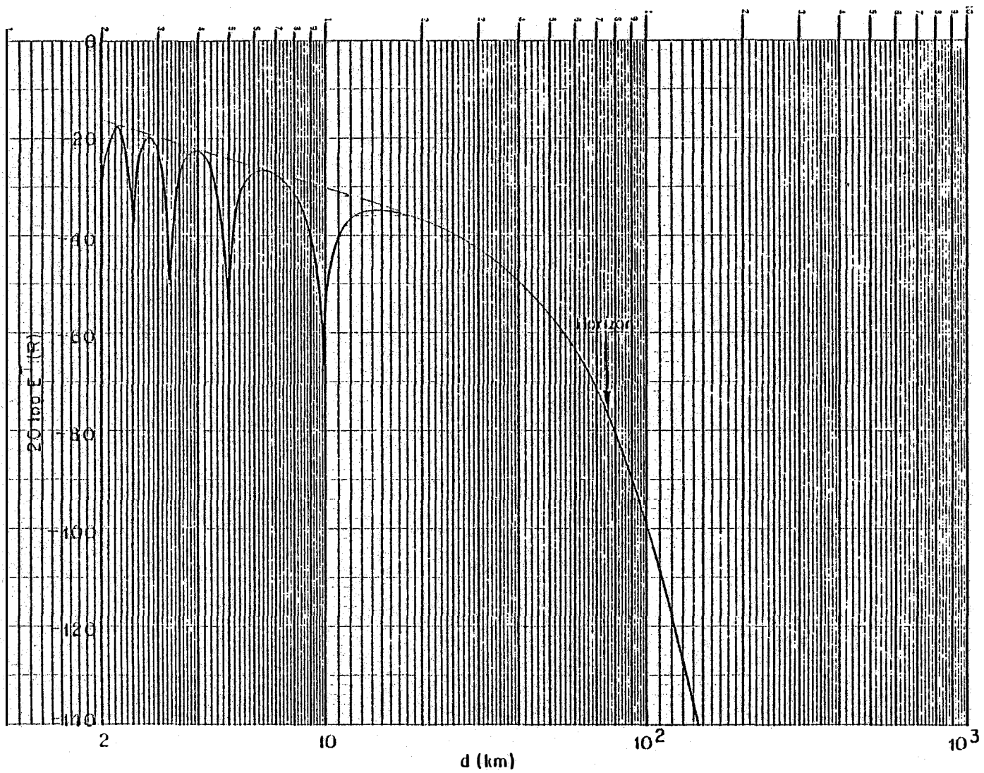
Figure 4. Field strength in dB above mv/m as a function of distance d from a horizontally polarized transmitter radiating 1 kw effective power: h_1 = 300 m, h_2 = 10 m, f = 500 MHz.
