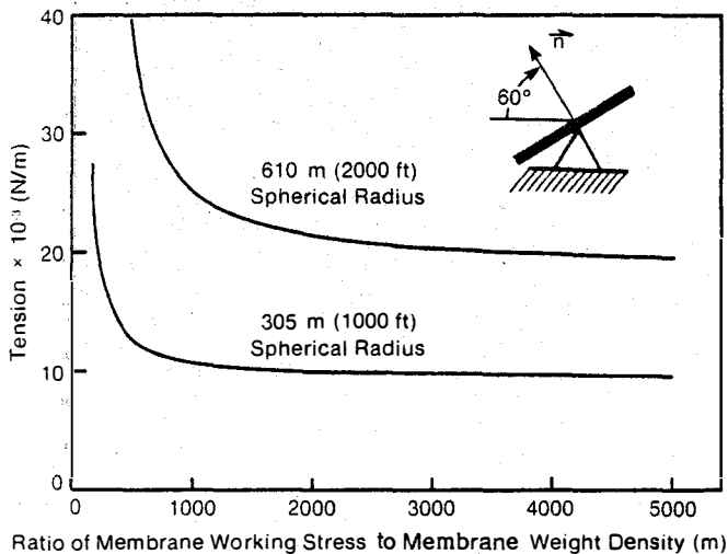
Fig. 8. REQUIRED MEMBRANE DESIGN TENSION AS A FUNCTION THE OPERATING STRESS AND WEIGHT RATIO.
