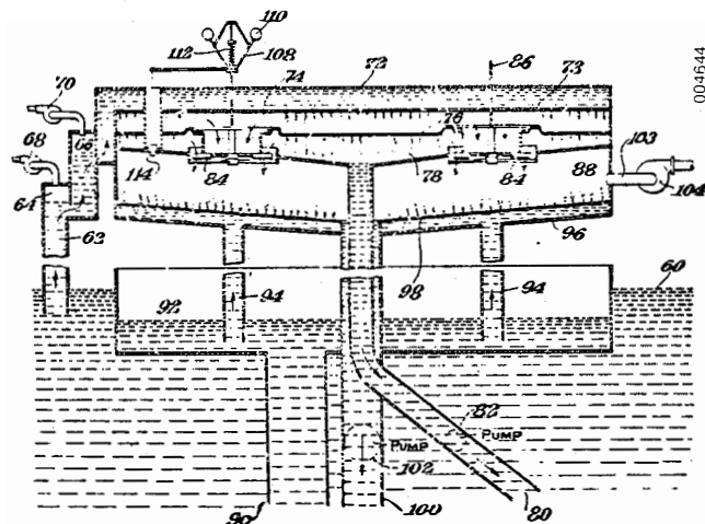
Fig. 1. Claude's 50-MW e Conceptual Open-Cycle Plant Design
